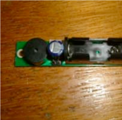
The altimeter: once the rocket was back on ground the altimeter will be heard to make an irregular beeping sound. These beeps tell you how high (apogee) the rocket reached; e.g. five beeps followed by two beeps followed by two beeps means that that rocket reached an apogee of 522 ft.
