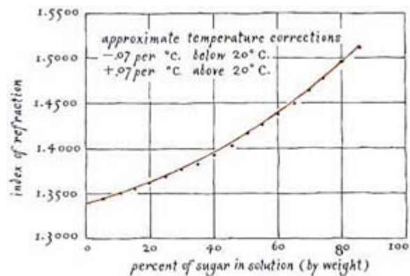
One student's results show a non-linear relationship for sugar but this is not what everyone gets.
