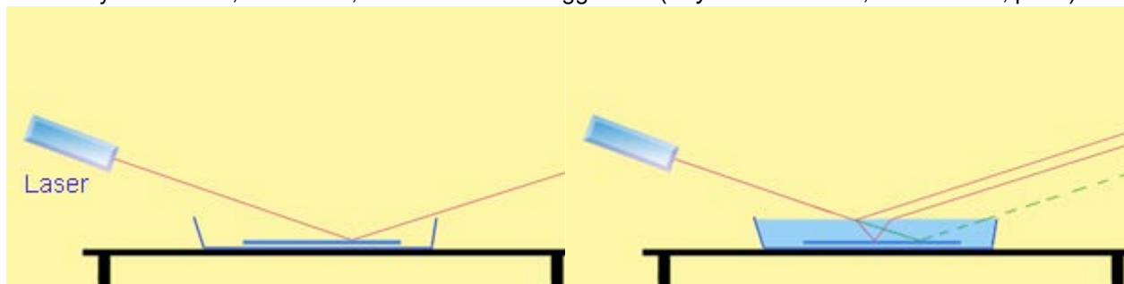
Firstly, without water. Clamp the laser in a stand and make sure the glass is dead level.
