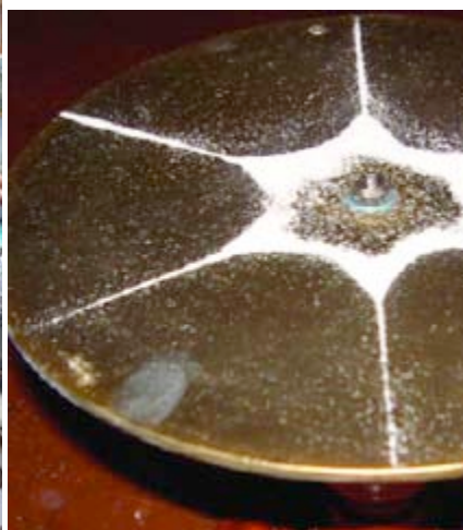
A simple Chladni pattern on a circular plate. Here the student has generated one with n=3 nodal lines and m=0 nodal circles.
