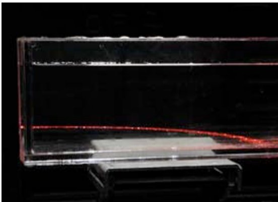
See how the laser beam bends down as it travels through a sugar solution with a high density at the bottom.
