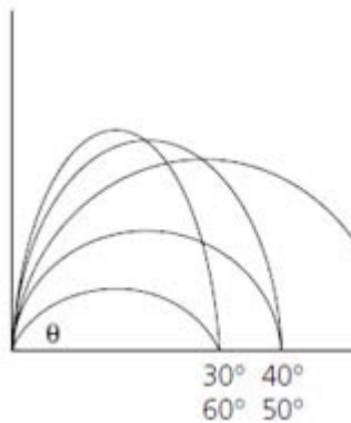
Theoretical path of a projectile (in a vacuum). Complementary angles seem to give the same range - but is this true in practice?
