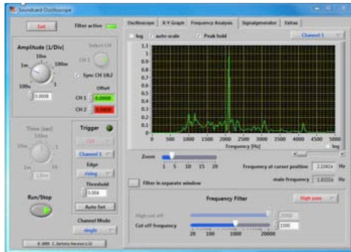
Here's a screen capture showing the fundamental frequency of a 1.200 m singing rod and a frequency of 2104 Hz. Click here to see a larger version plus some notes.
