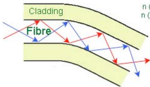
Shallow bend
