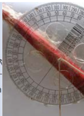
A protractor stuck to the bow and with a brass bob hanging down is one way of measuring the elevation angle.
