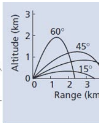
In air the path is somewhat different. This is for a cannon shell going to great heights - not an arrow.
